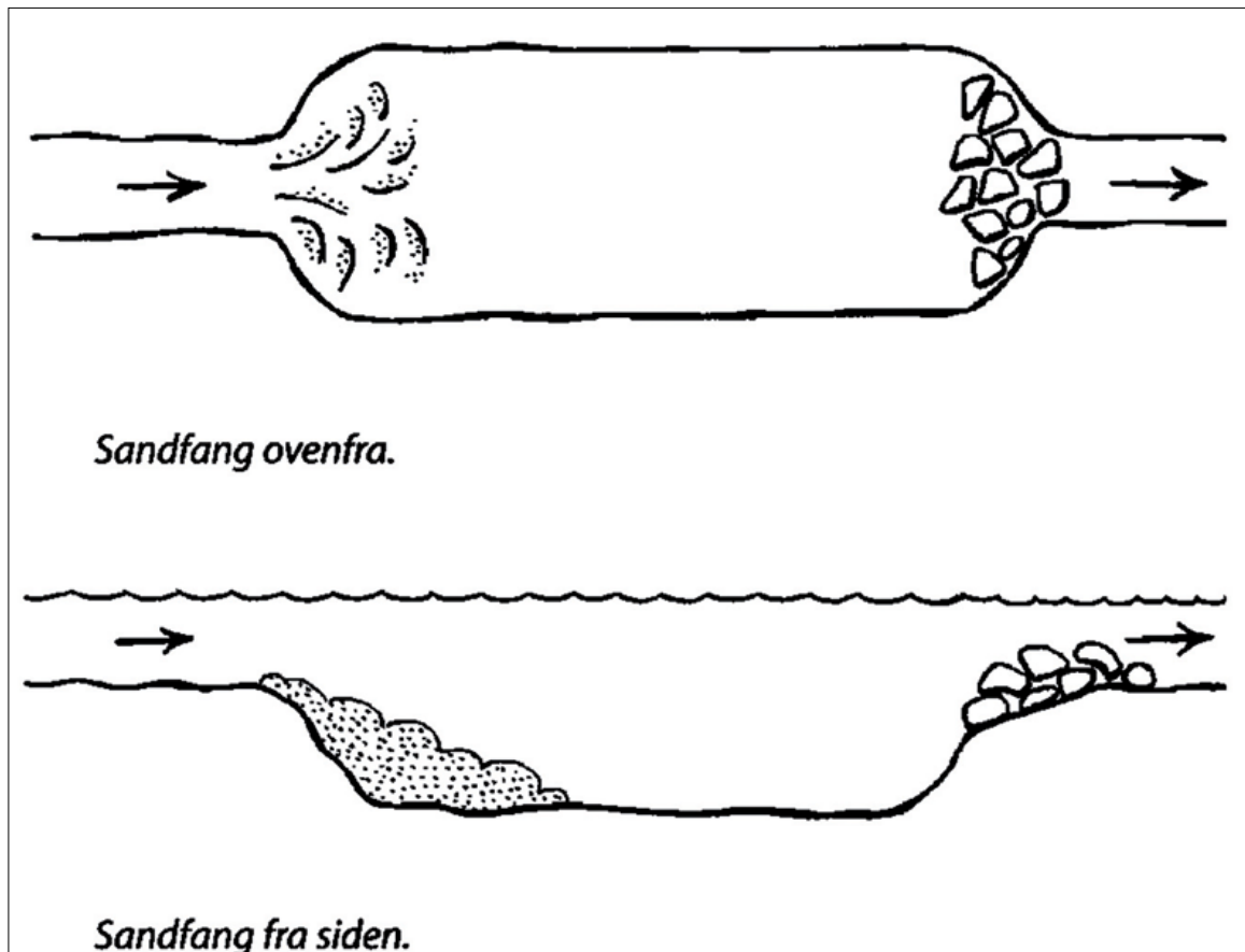
Figur 2: Principskitse for sandfang.
